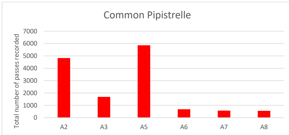
Plate 8-49: Total number of bat passes recorded for Common pipistrelles at each of the static detector locations in 2020.
