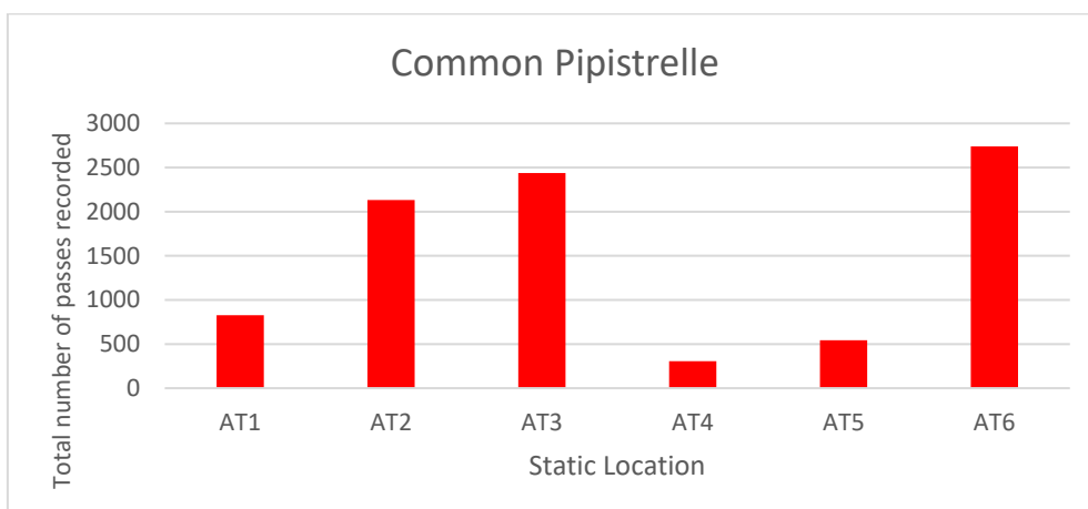
Plate 8-59: Total number of bat passes recorded for common pipistrelle at each of the static detector locations during 2020.
