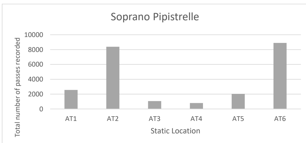
Plate 8-60: Total number of bat passes recorded for soprano pipistrelles at each of the static detector locations during 2020.
