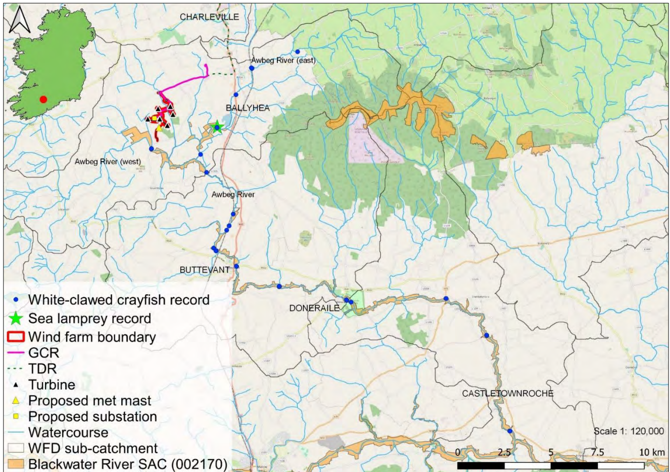
Plate 8-63: Distribution of selected protected aquatic species in the vicinity of the survey area
