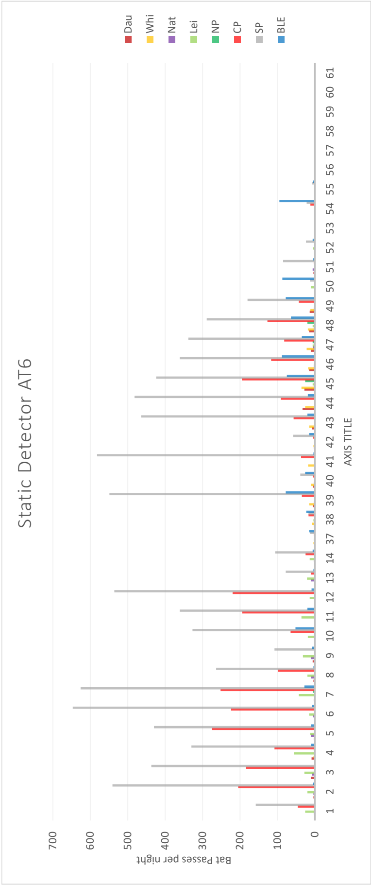
Plate 8-58: Total number of nightly bat passes recorded at static location AT6
