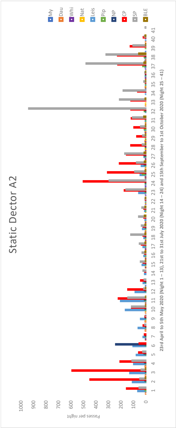
Plate 8-43: Total number of nightly bat passes recorded at Static location A2
