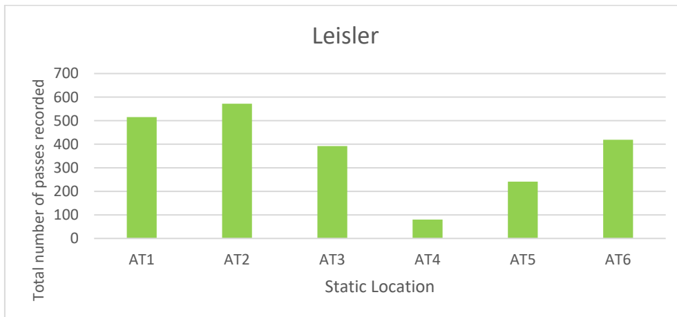
Plate 8-61: Total number of bat passes recorded for leisler's bat at each of the static detector locations during 2020
