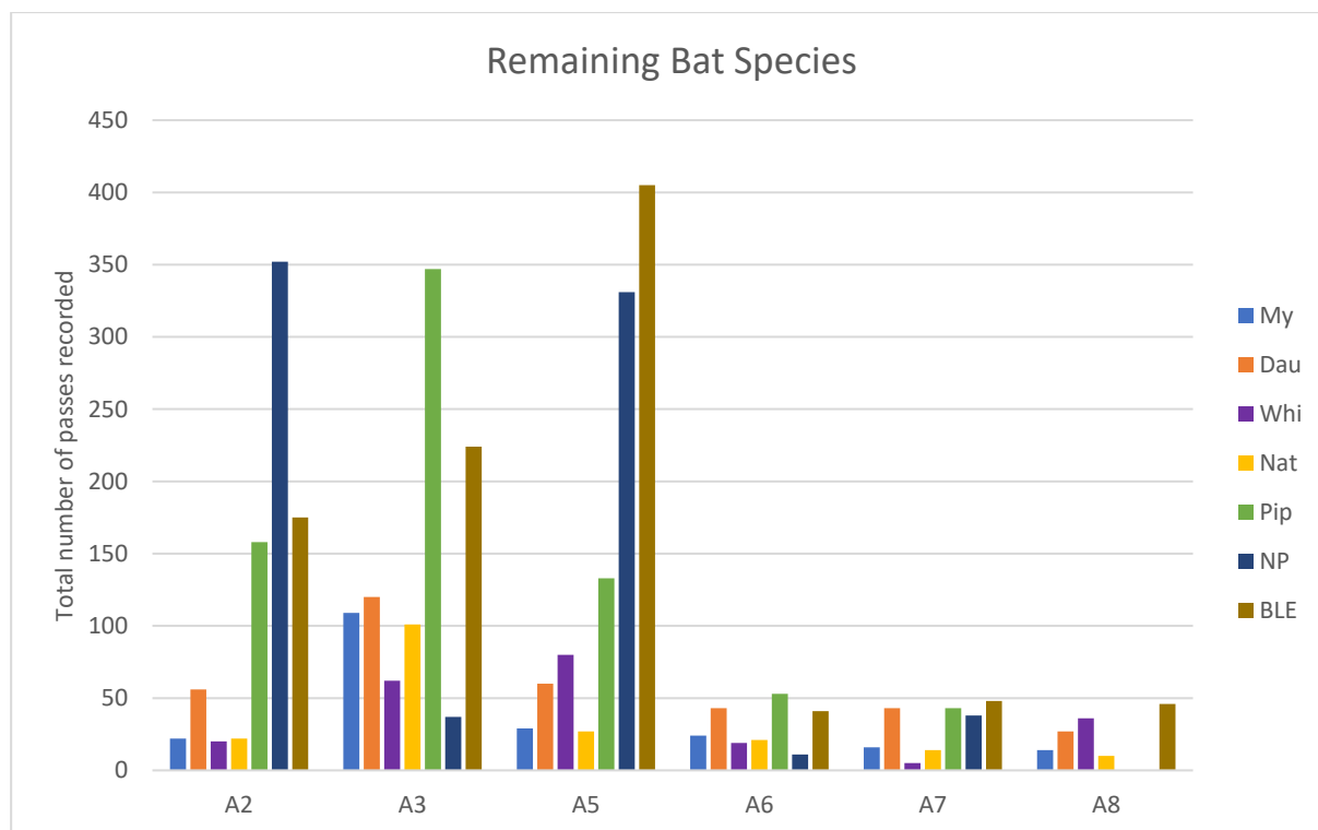
Plate 8-52: Total number of bat passes recorded for remaining bat species at each of the static detector locations in 2020.
