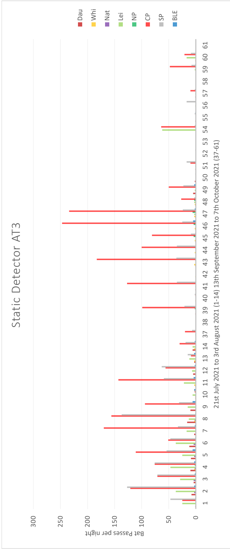
Plate 8-55: Total number of nightly bat passes recorded at static location AT3
