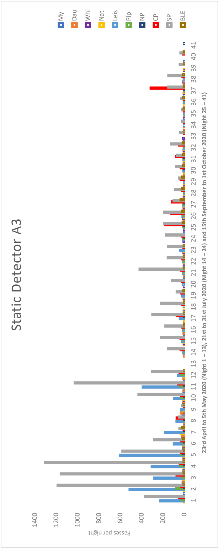
Plate 8-44: Total number of nightly bat passes recorded at Static location A3
