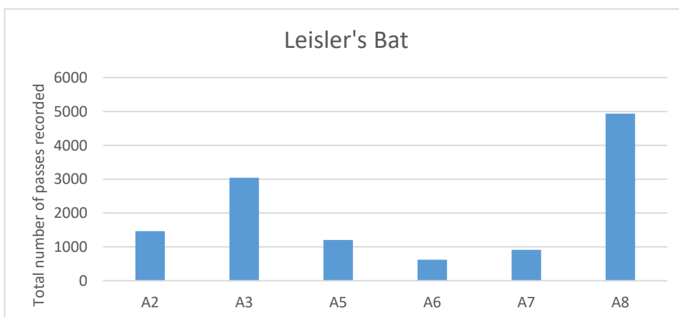
Plate 8-51: Total number of bat passes recorded for Leisler's bat at each of the static detector locations in 2020.
