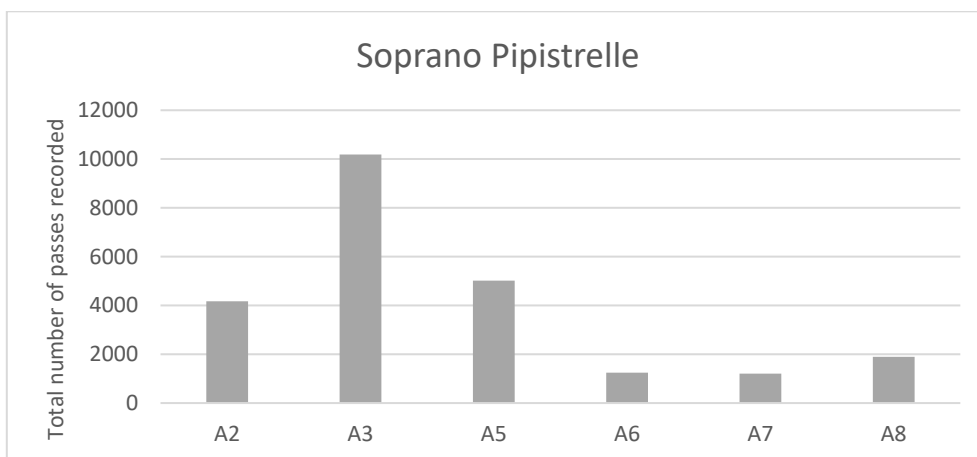
Plate 8-50: Total number of bat passes recorded for Soprano pipistrelles at each of the static detector locations in 2020.
