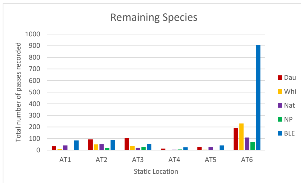
Plate 8-62: Total number of bat passes recorded for remaining bat species at each of the static detector locations in 2020.
